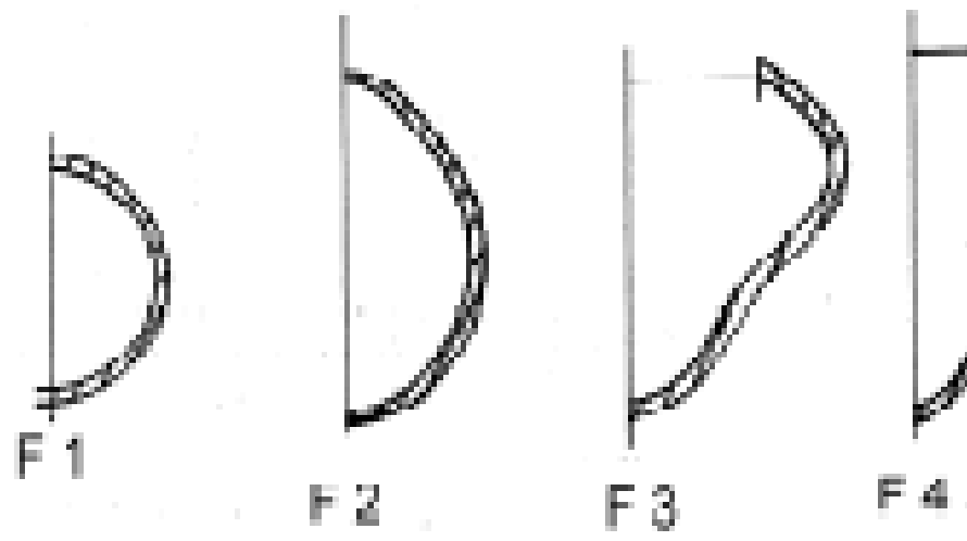
Nose cone formers (3mm depth)
